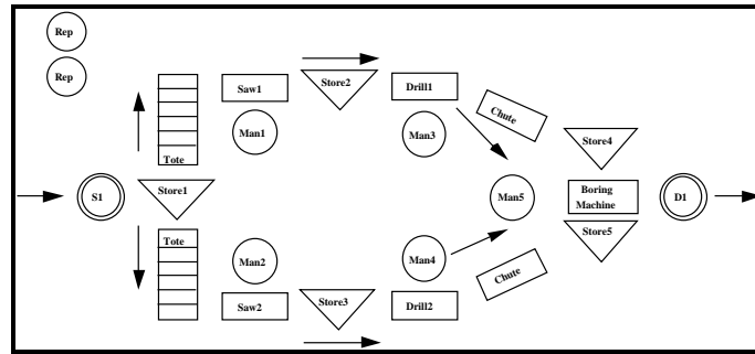
Figure A-9. Facility Submodel used for Plant Layout
