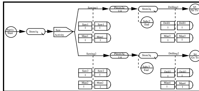
Figure A-10. Example Entity Flow Network
